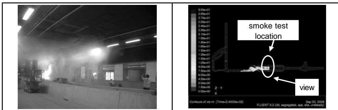
Figure 4: Hot smoke test image compared to CFD result of smoke spread
